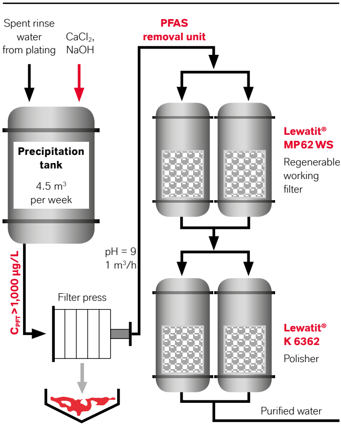
Figure 1: Flow sheet describing a pilot plant setup for the removal of PFAS from plating baths. Lewatit® MP 62 WS acts as a regenerable working filter, removing the main part of PFAS. Lewatit® K 6362 polishes the water and enables our customers to comply with wastewater limits.
