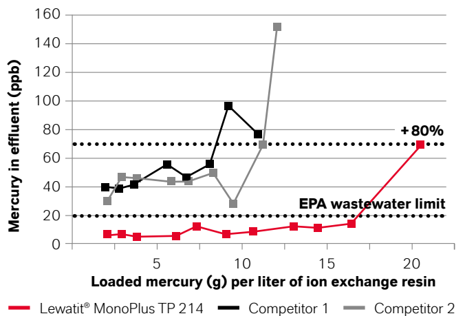
Figure: Breakthrough curves depicting the mercury concentration determined by inductively coupled plasma spectrometry in the effluent of the ion exchange column depending on the amount of mercury loaded on the resin.
